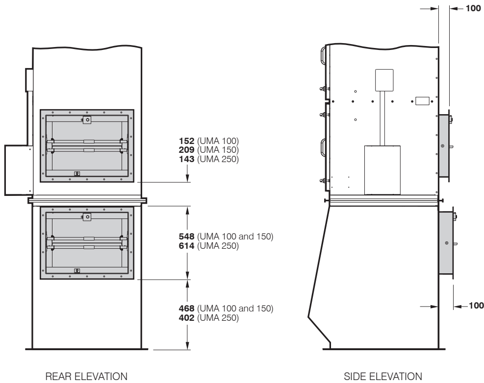
POSITION OF OPTIONAL EXPLOSION RELIEF FLANGES FOR SACK TIPPING UNITS UMA 150STU illustrated
