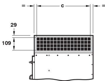
SIDE ELEVATION (Detail of cleaned air outlet with weather cowl and lid removed)
