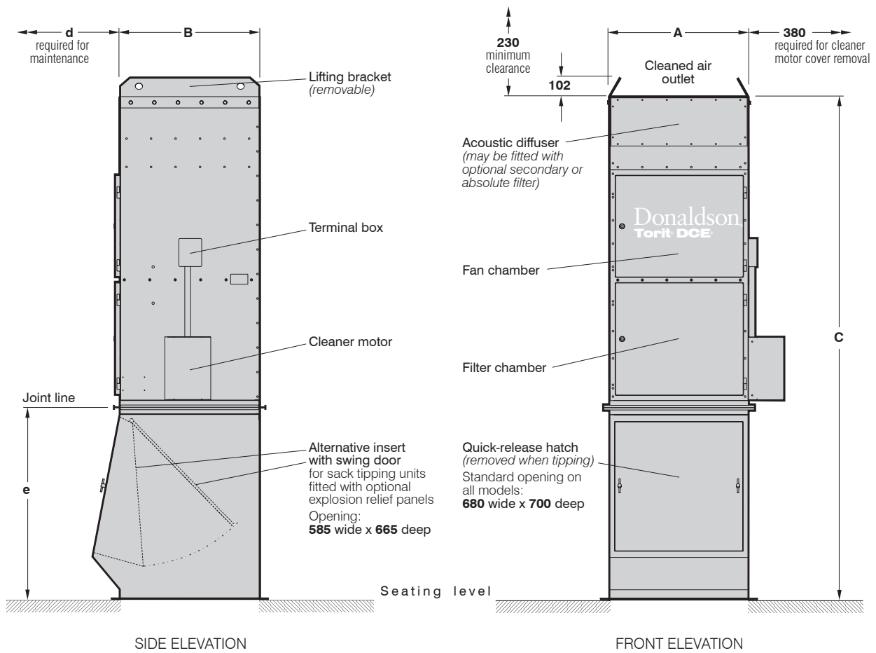
UNIMASTER SACK TIPPING UNIT UMA 150STU illustrated. Suitable for inside locations.
