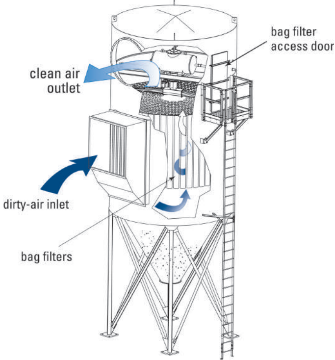
Normal Operation with High Body Inlet
