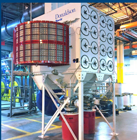
Flameless Explosion Vent
